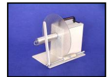
MC-10A (right): You can use the included 3-inch core holder, or rewind "coreless" directly "on-shaft" without any label core as set up in the photo below. Also shown below is the Optional APG-MC Adjustable Paper Guide.
