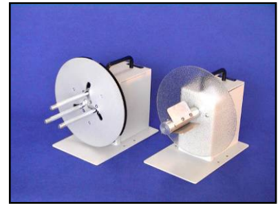
MC-11 (left): Rewind on any core from 1" to 4" diameter, or coreless.
